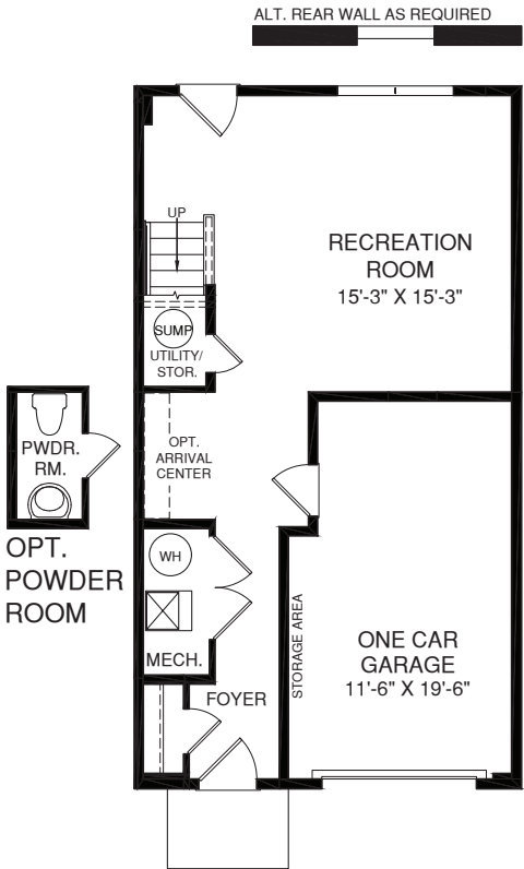
LOWER LEVEL
