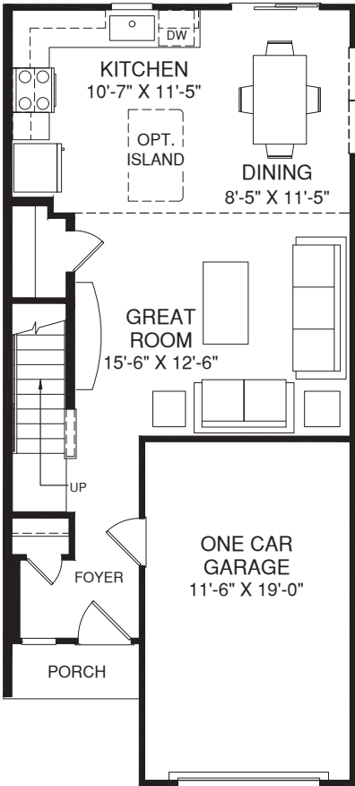
MAIN LEVEL
