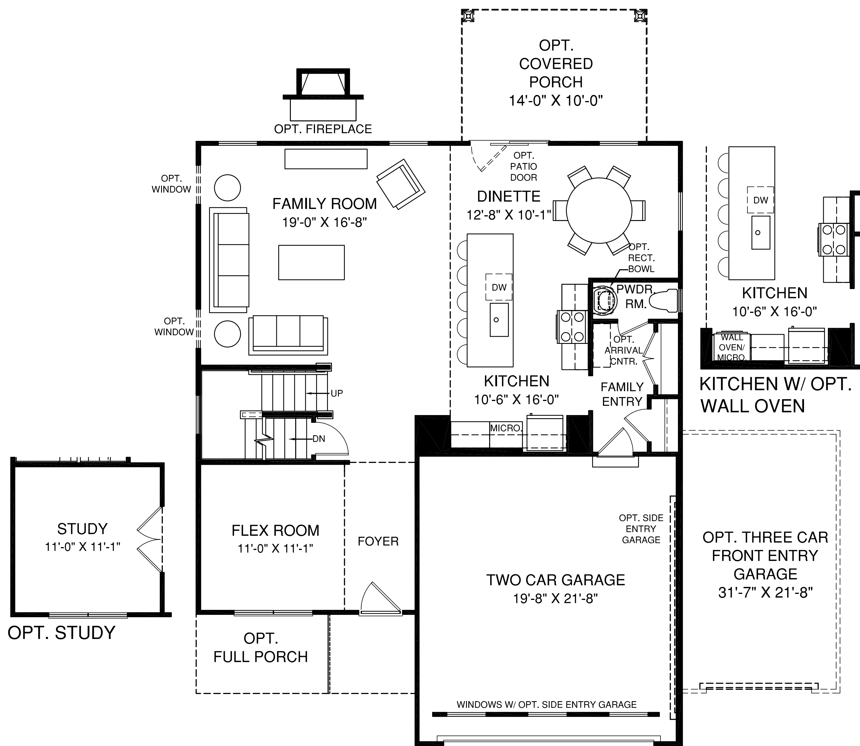
MAIN LEVEL
