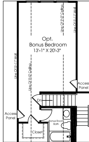
Opt. Bonus Bedroom W/ Rear Attached Garage
