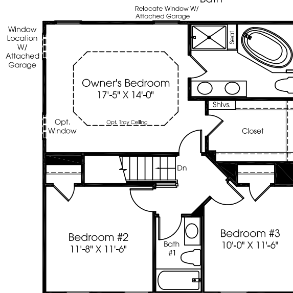
Second Floor W/ Three Bedrooms
