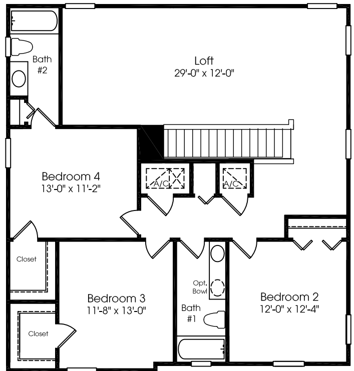
Second Floor w/ Opt. Fourth Bedroom and Loft
