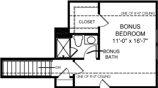
OPT. BONUS BEDROOM W/ OPT. MORNING ROOM
