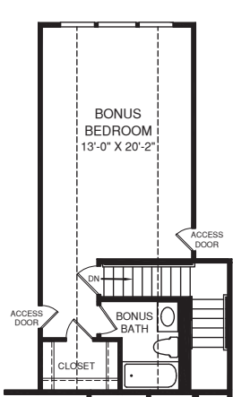
OPT. BONUS BEDROOM
