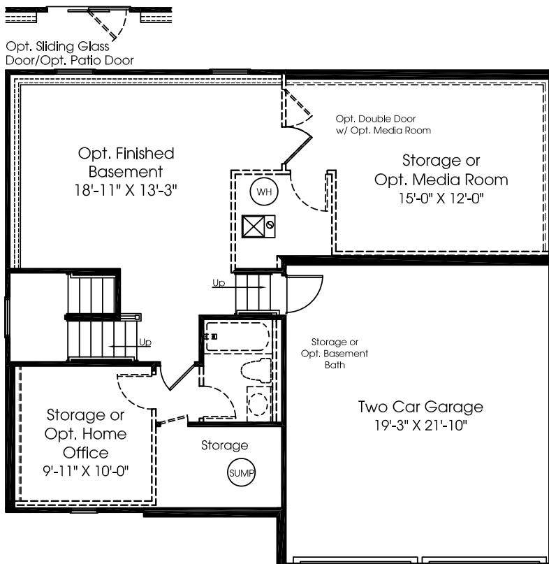
Opt. Finished Basement w/ Opt. Morning Room
