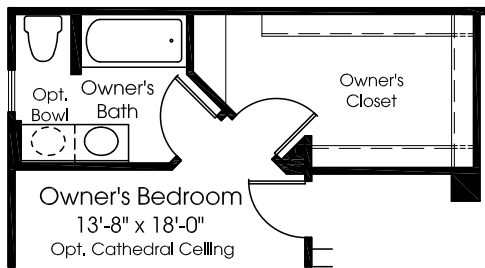
Owner's Bedroom w/ Opt. 4' Ext. @ Great Room
