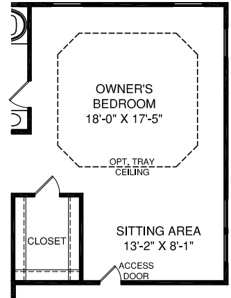
OWNER'S BEDROOM w/ OPT. SITTING ROOM
