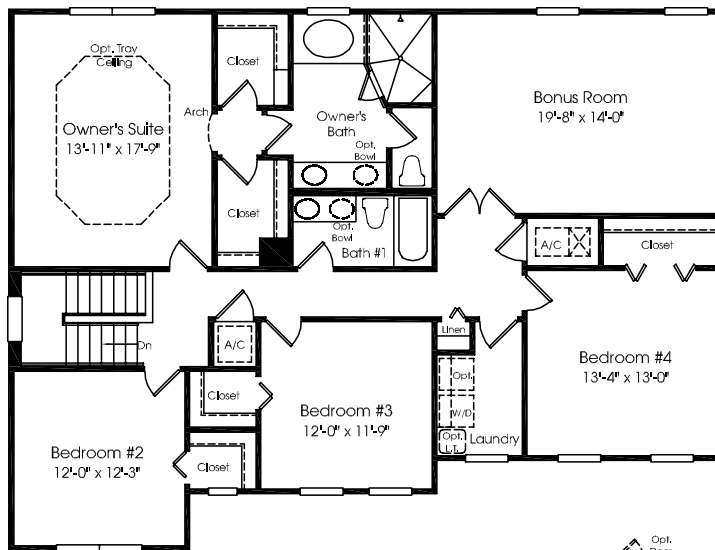
Opt. Alternate Owner's Suite
