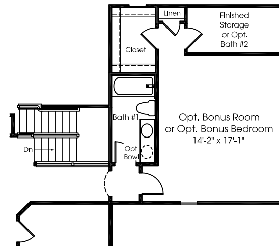
Second Floor w/ Opt. Bonus Room or Opt. Bedroom
