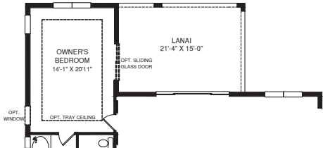
OPT. 4'-0" EXTENSION AT OWNER'S BEDROOM
