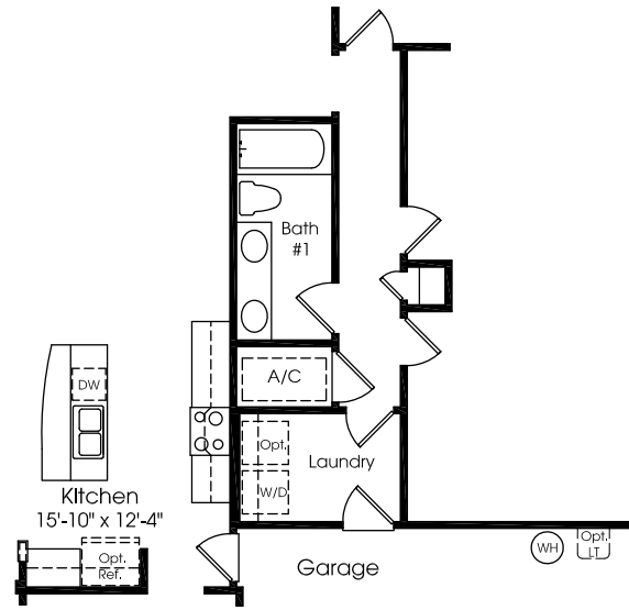
Opt. Bath 1 Layout
