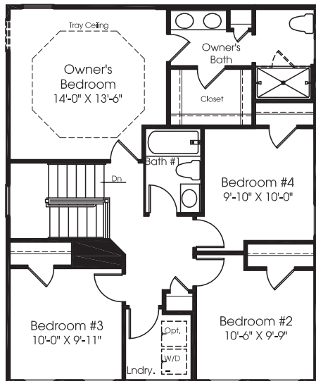
Second Floor W/ Four Bedroom Opt.
