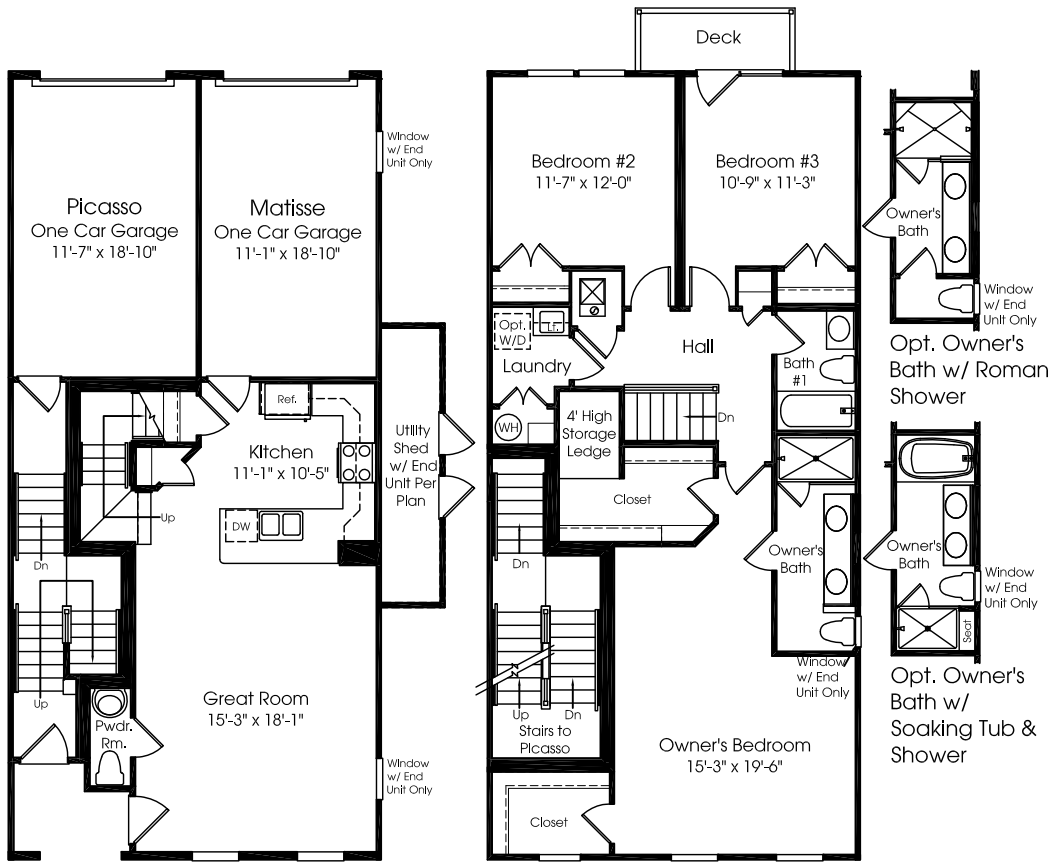
First Floor Matisse Main Level
