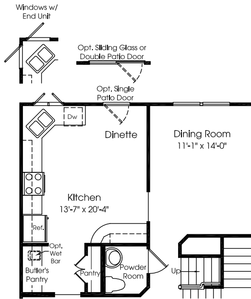
First Floor w/ Formal Dining Room & Opt. 4' Ext.
