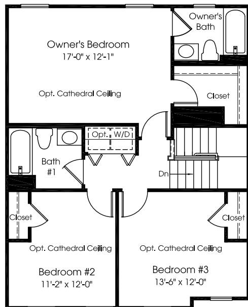
Second Floor w/ 3 Bedrooms & 2 Baths
