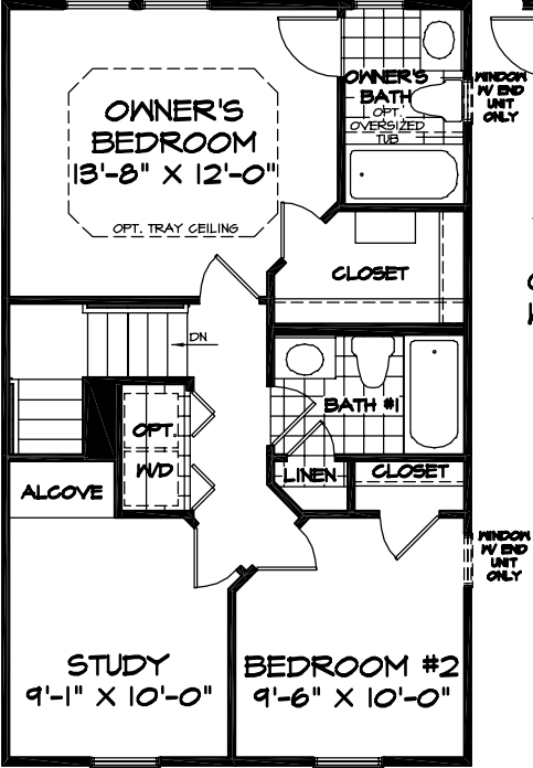
SECOND FLOOR W/ OPT. OWNER'S BATH
