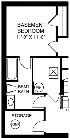
OPT. BASEMENT BEDROOM
