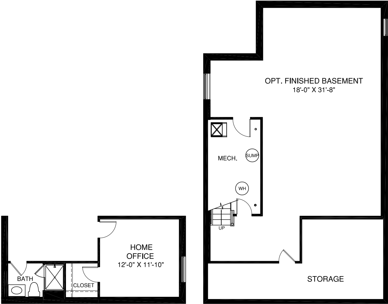
OPT. HOME OFFICE AND OPT. BSMT BATH
