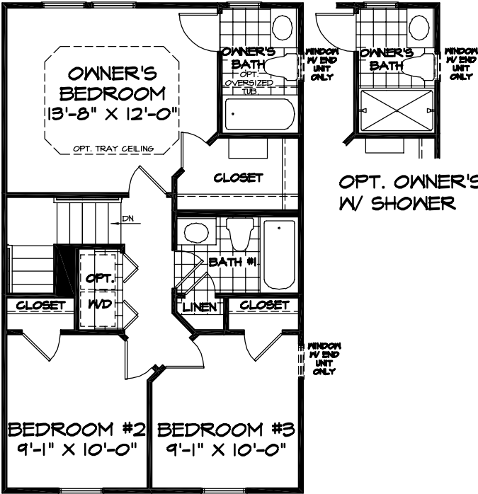
SECOND FLOOR W/ OPT. OWNER'S BATH
