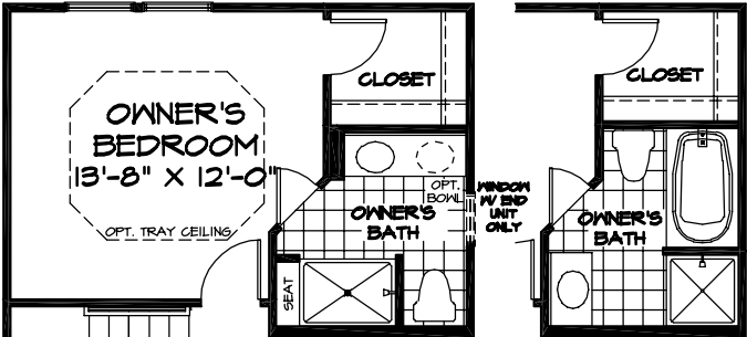
OPT. OWNER'S BATH W/ SEPARATE SOAKING TUB AND SHOWER
