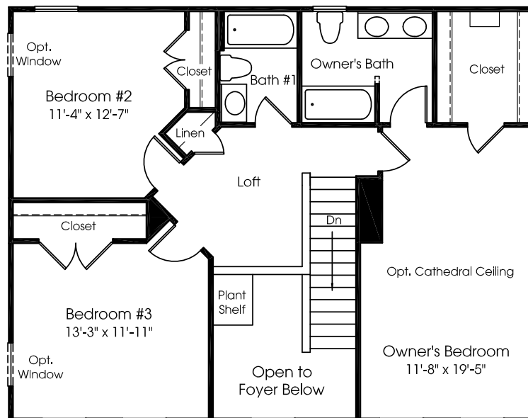
Second Floor w/ 3 Bedrooms
