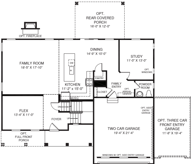
MAIN LEVEL
