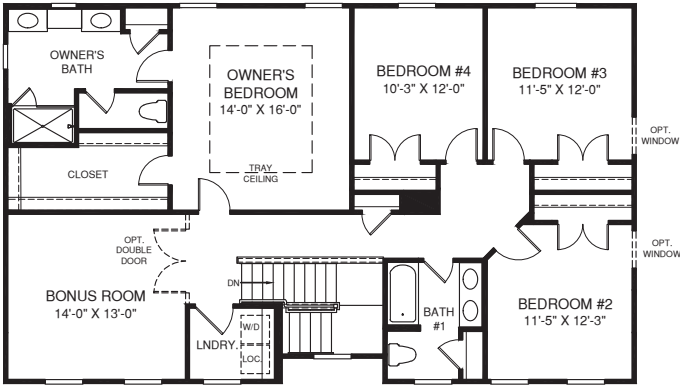
OPT. FOUR BEDROOMS W/ BONUS ROOM
