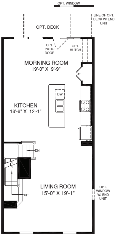
MAIN LEVEL
