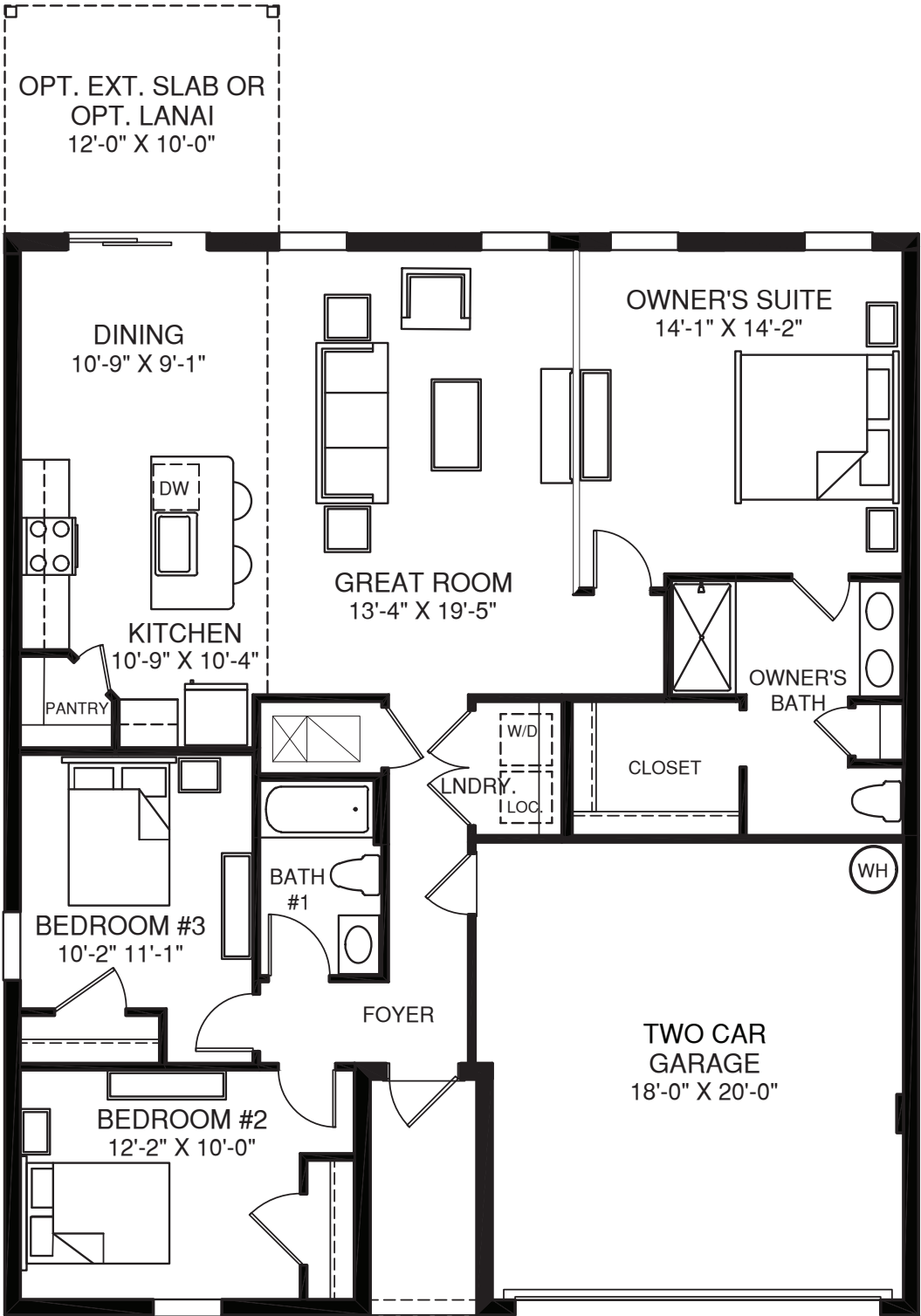
MAIN LEVEL
