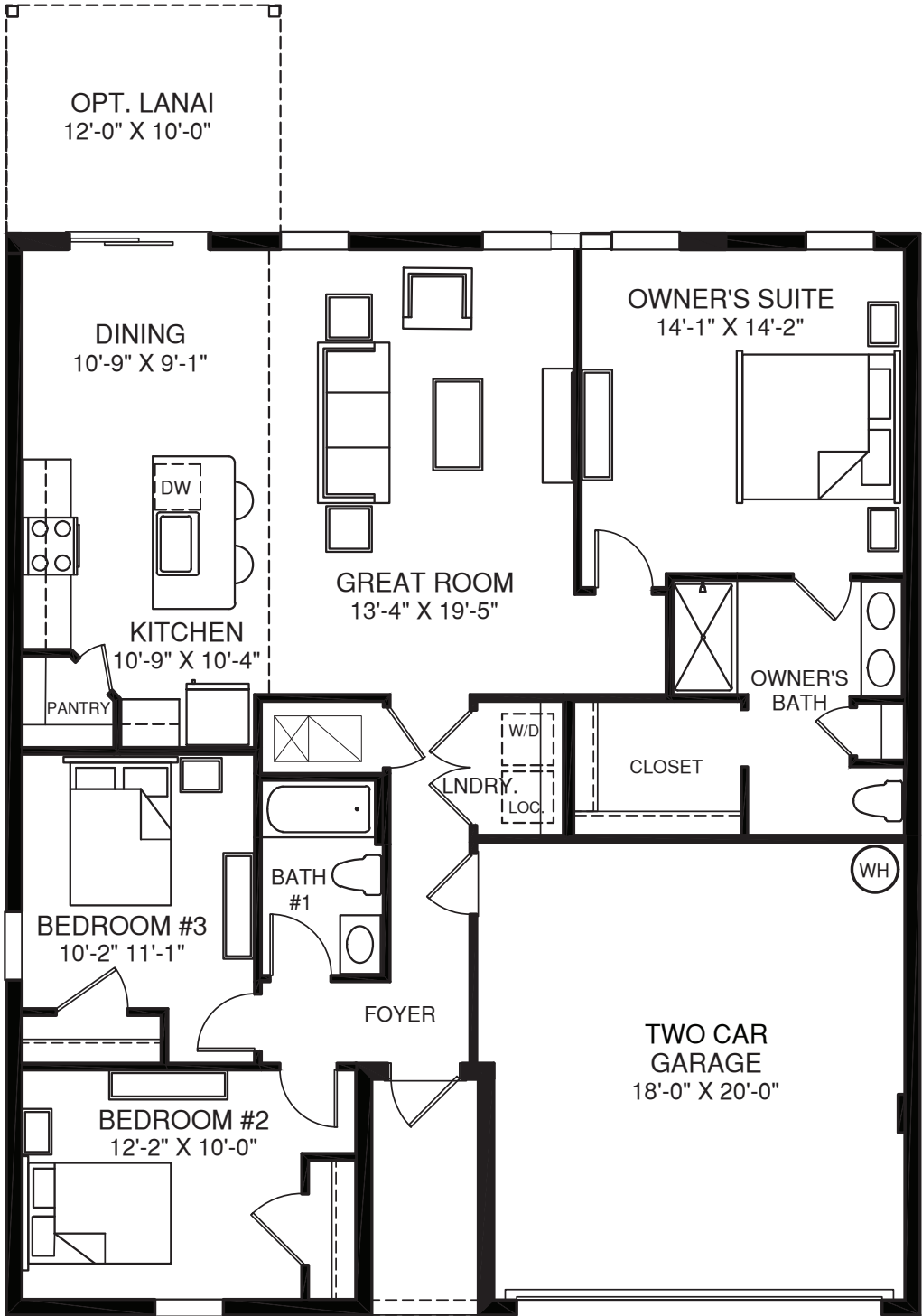
MAIN LEVEL
