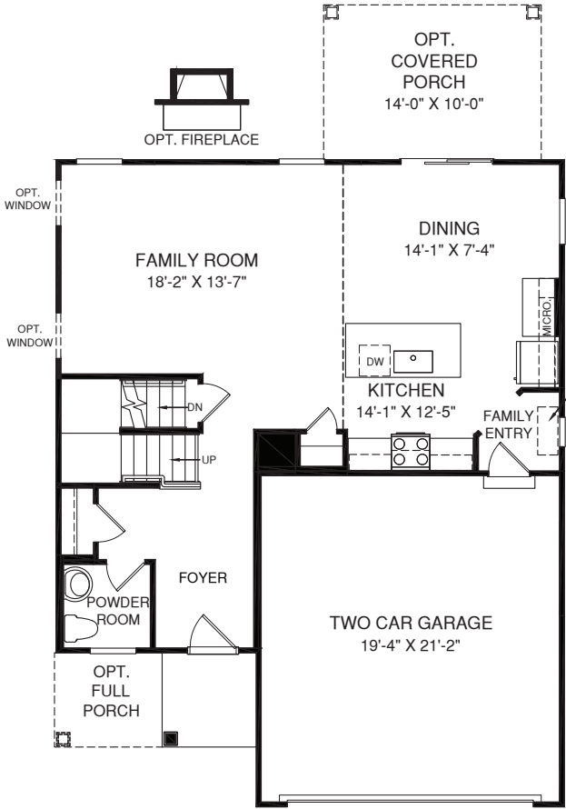
MAIN LEVEL
