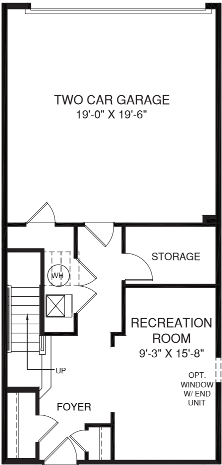
LOWER LEVEL
