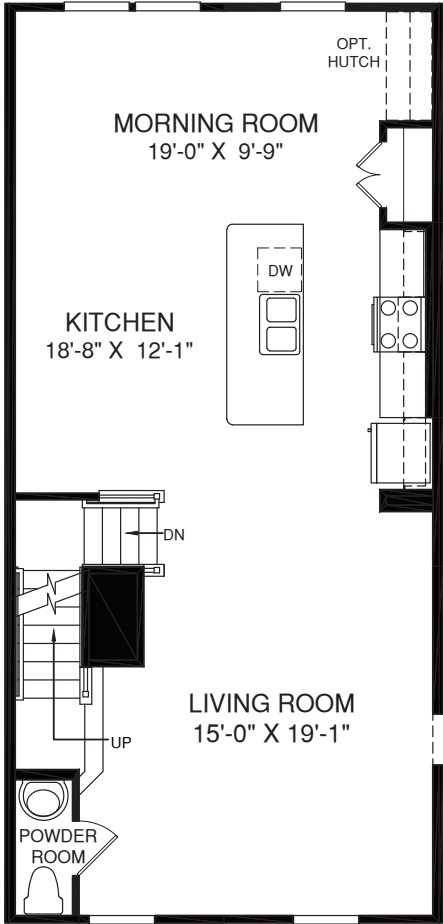
MAIN LEVEL
