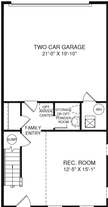
LOWER LEVEL
