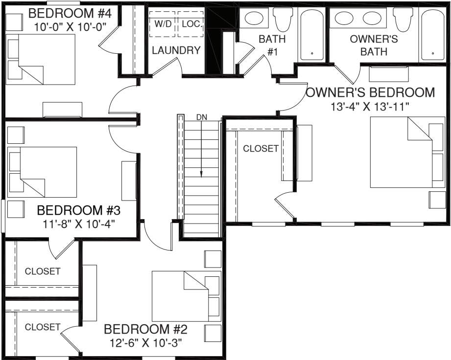
UPPER LEVEL
