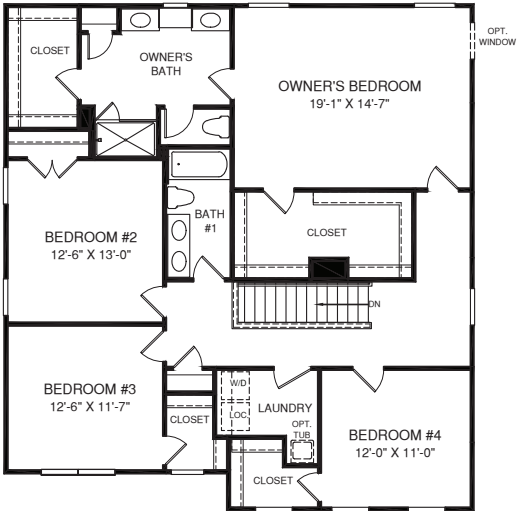
UPPER LEVEL
