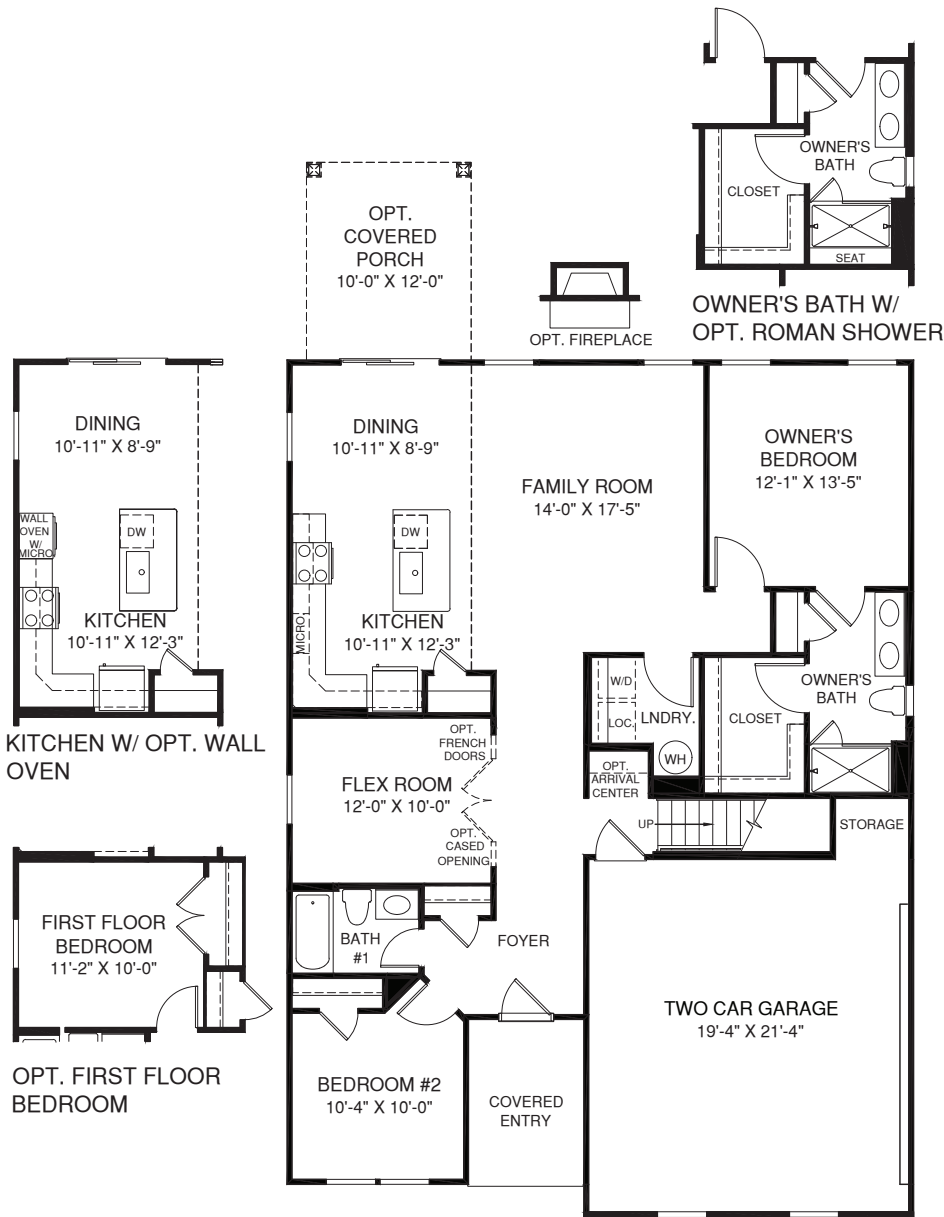
MAIN LEVEL
