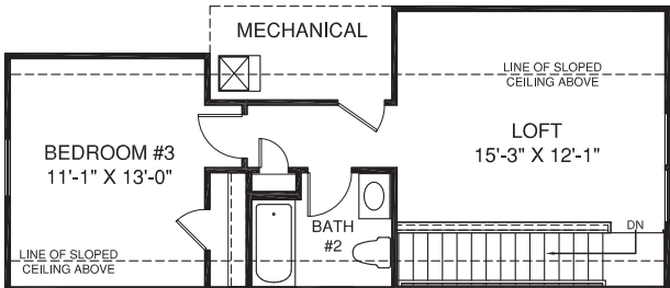
UPPER LEVEL
