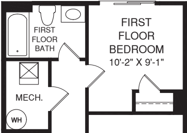
OPT. FIRST FLOOR BEDROOM
