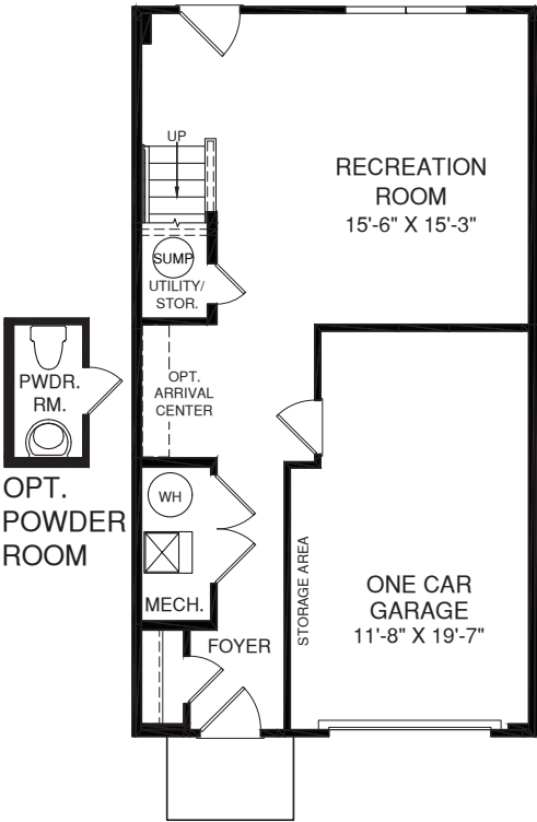
LOWER LEVEL
