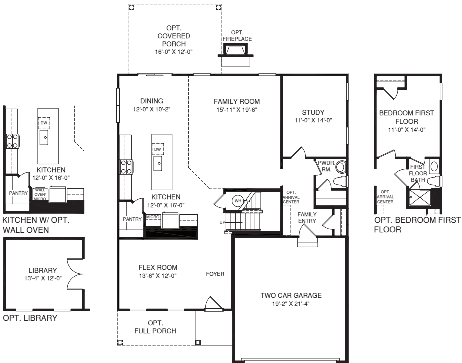
MAIN LEVEL
