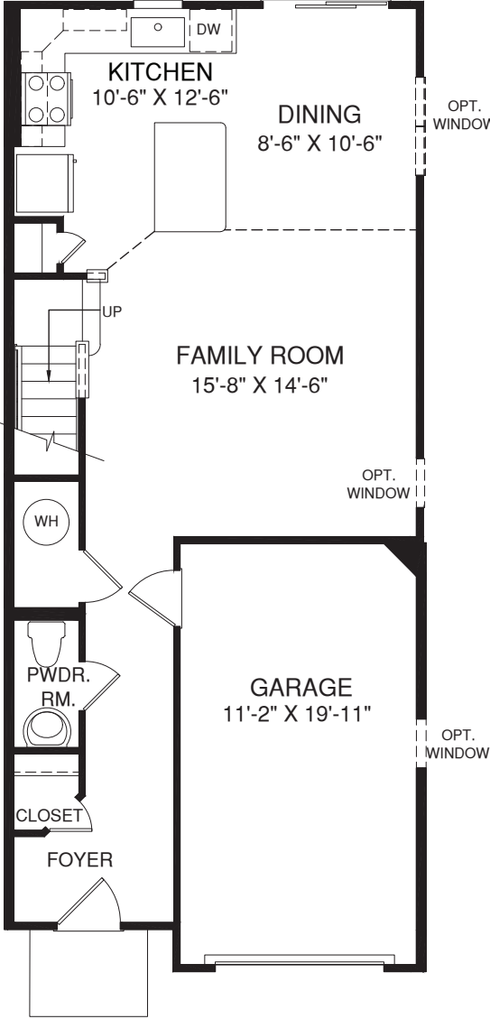
MAIN LEVEL
