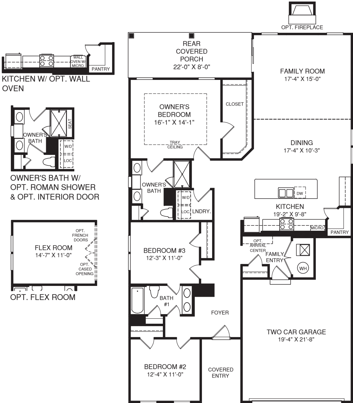
MAIN LEVEL
