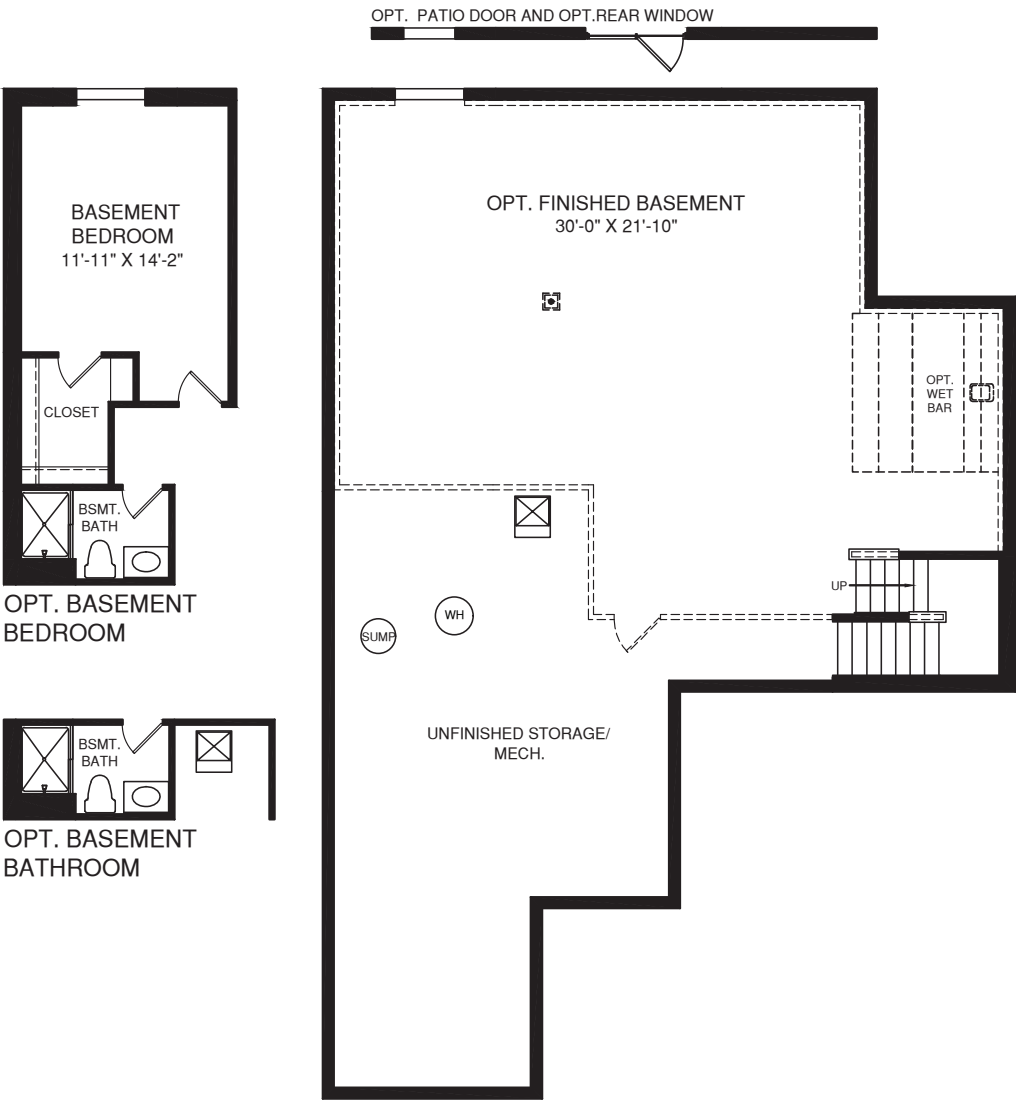
LOWER LEVEL
