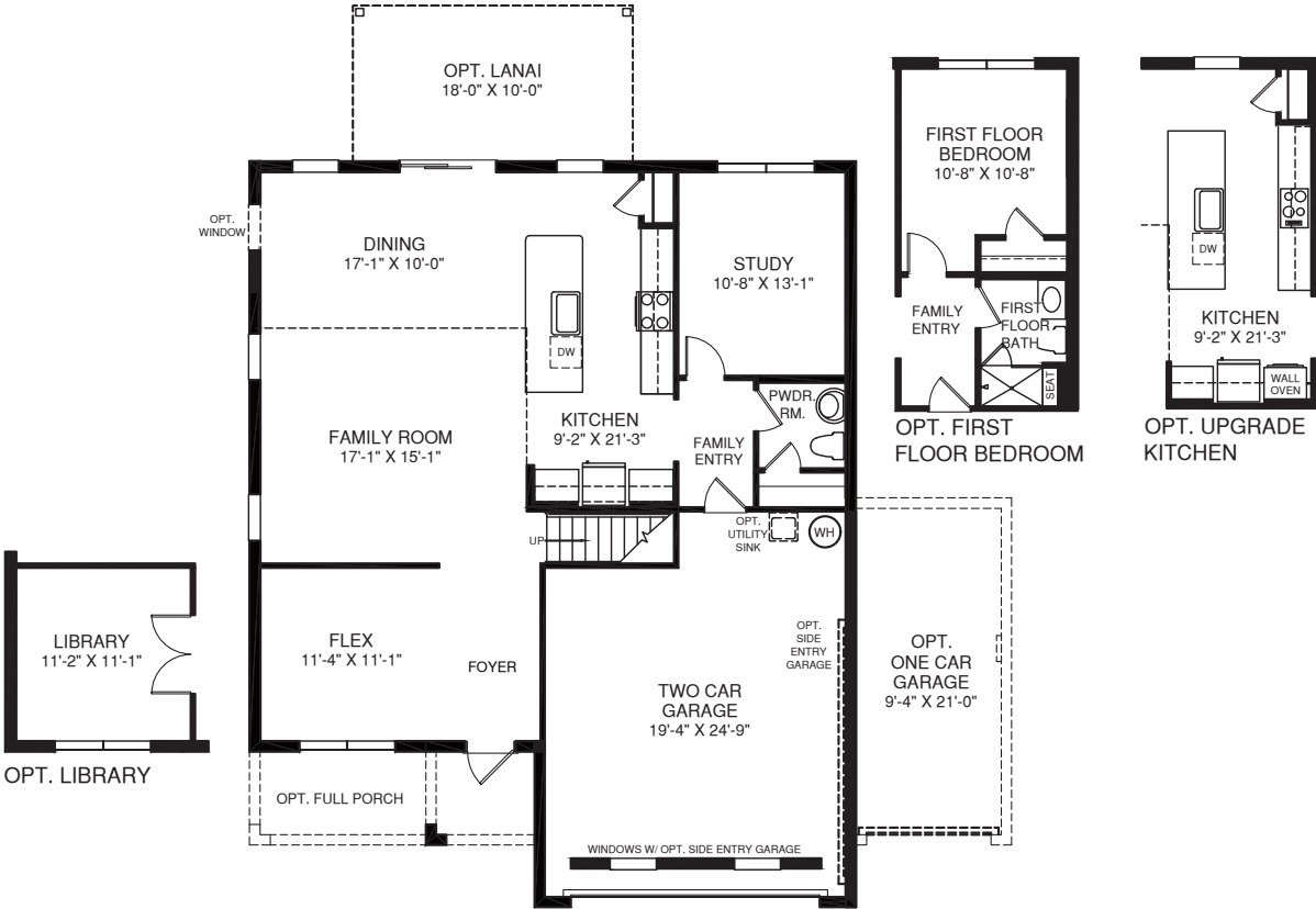
MAIN LEVEL
