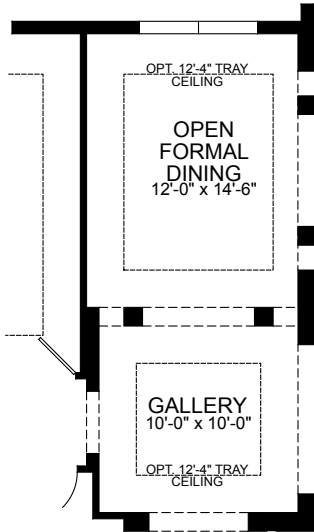
OPT. OPEN FORMAL DINING
