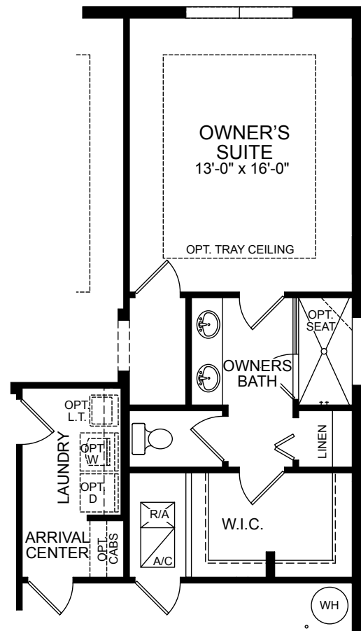
OPT. ALT LAUNDRY & OWNER'S BATH
