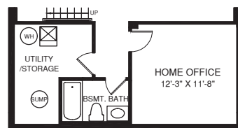
OPT. HOME OFFICE SHOWN W/ OPT. BASEMENT BATH
