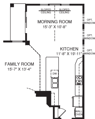
OPT. MORNING ROOM SHOWN W/ OPT. UPGRADE KITCHEN (MORNING ROOM NOT AVAILABLE WITH REAR ATTACHED GARAGE)
