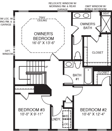
OPT. OWNER'S BATH W/ SOAKING TUB & SHOWER
