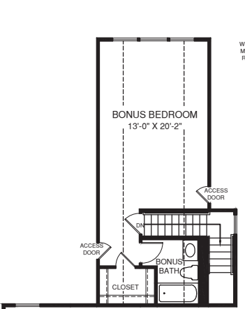
OPT. BONUS BEDROOM (ONLY AVAILABLE WITH OPT. REAR ATTACHED GARAGE)
