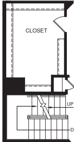
LAYOUT W/ OPT. 4TH FLOOR
