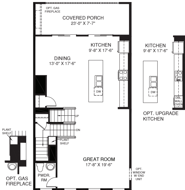
MAIN LEVEL
