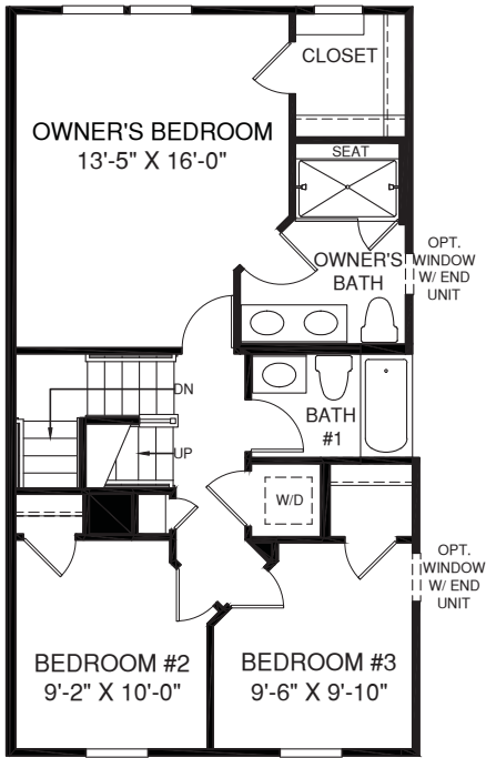
UPPER LEVEL
