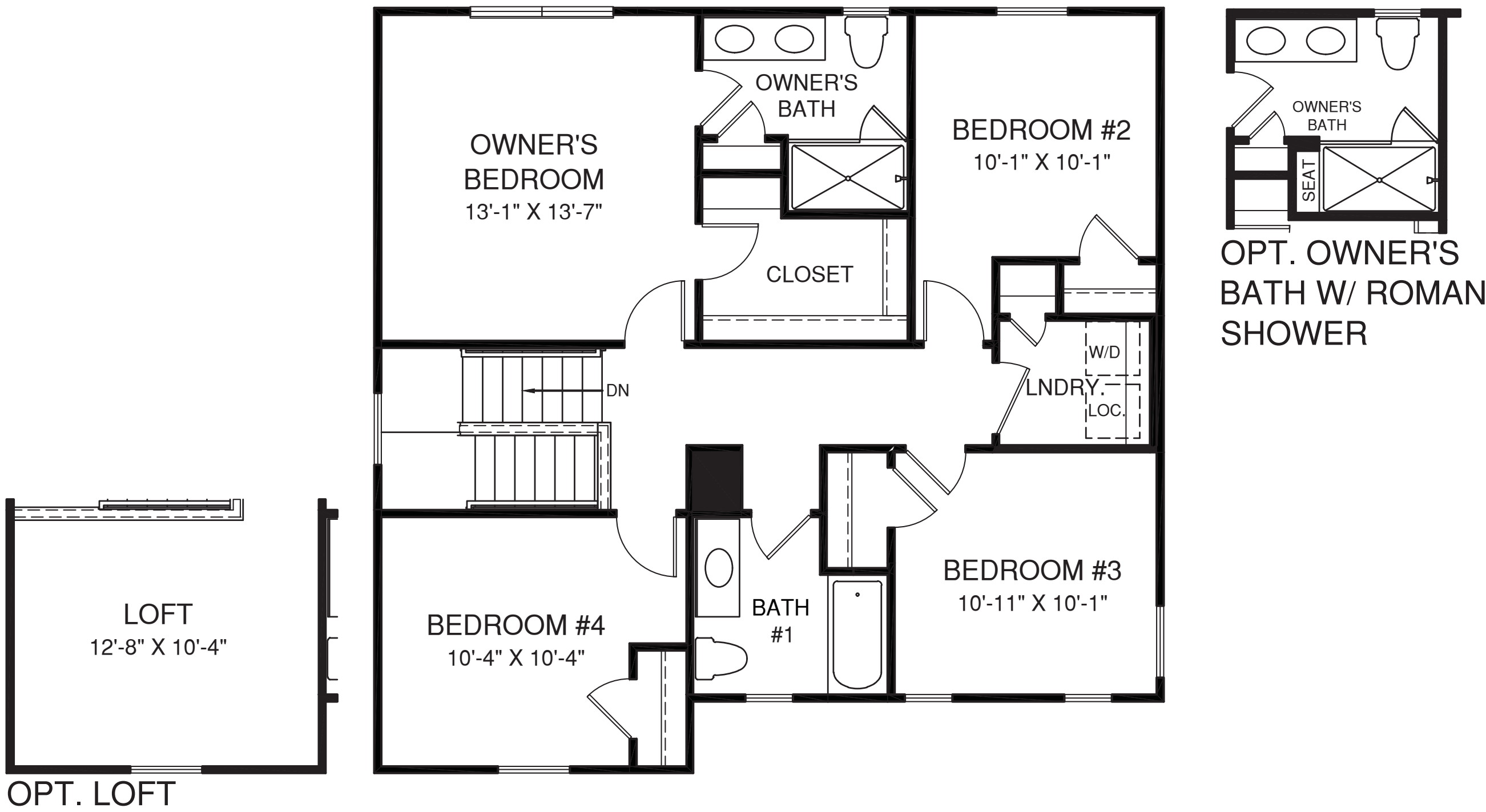
UPPER LEVEL
