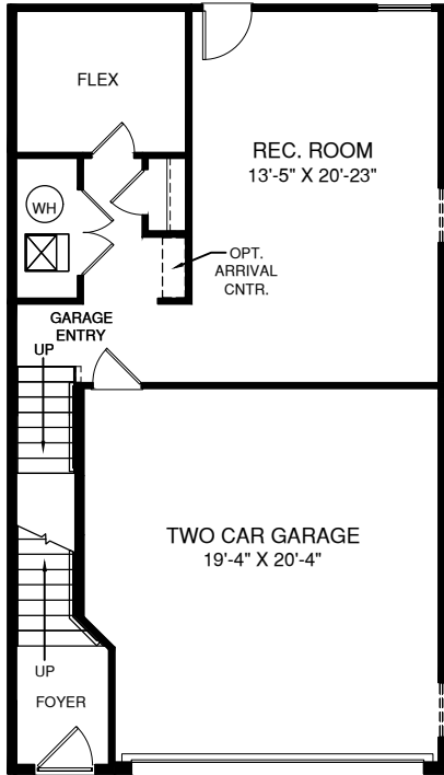
OPT. 4'-0" EXTENSION TO HOUSE
