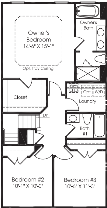
UPPER LEVEL
