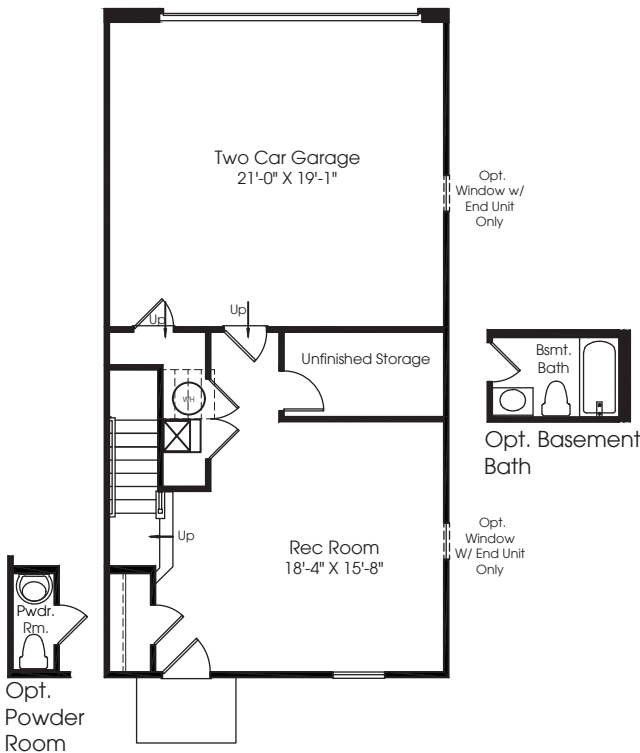
LOWER LEVEL
