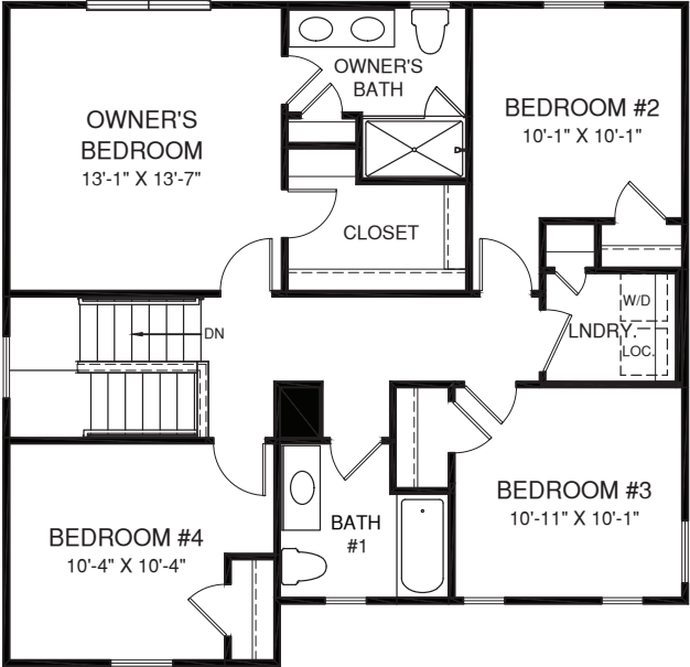
UPPER LEVEL
