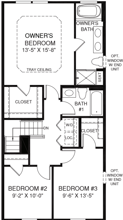
UPPER LEVEL
