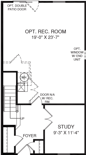
LOWER LEVEL
